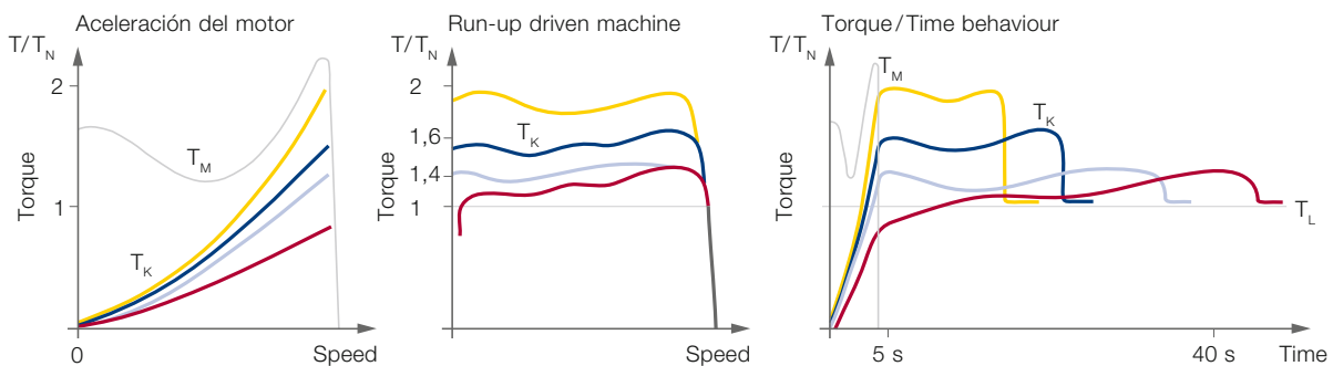
Characteristic curves
