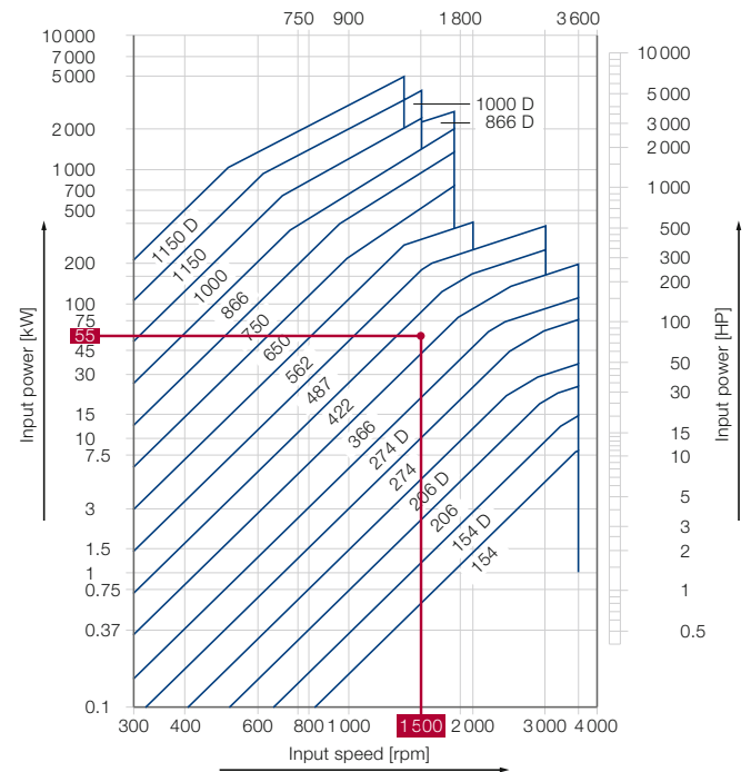
Performance diagram
