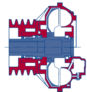
Type TVRI
