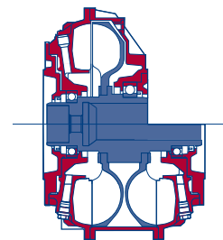
Type DT
